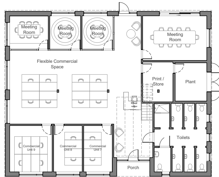
Commercial Units Building 2 Ground Floor Total GIA: 250m 2
