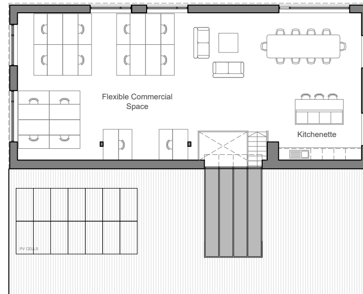
Commercial Units Building 2 First Floor Total GIA: 135m 2
