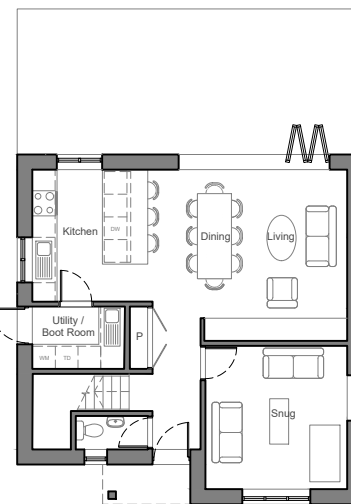
Type B2 Ground Floor GIA: 65m 2
