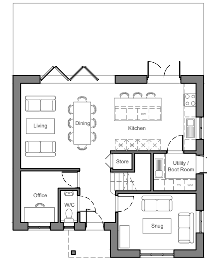
Type B1 Ground Floor GIA: 75m 2
