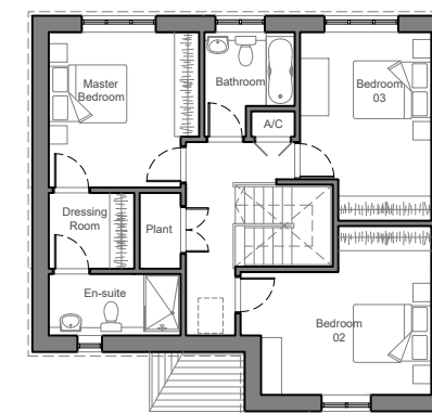
Type B1 First Floor GIA: 75m 2
